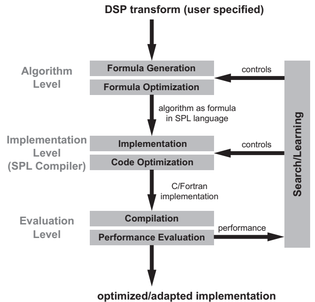
Fig. 1. The architecture of SPIRAL.
