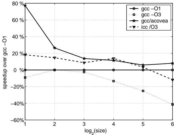
(a) improvement from compiler options search for DCT-2 of sizes 2^1, \dots, 2^6 .
