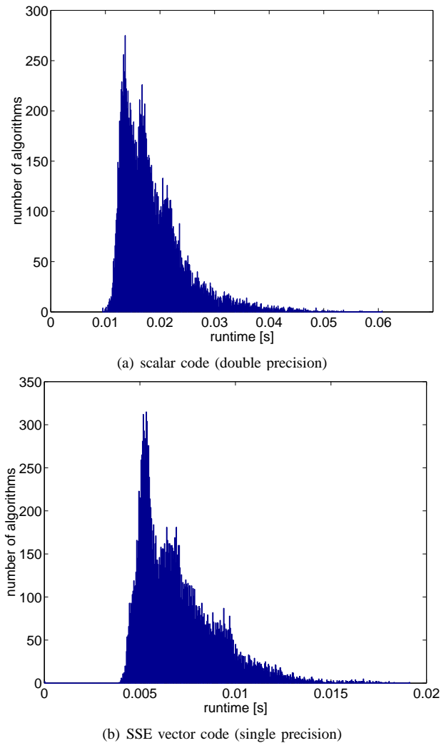
Fig. 9. Histogram of 20,000 random SPIRAL generated scalar and SSE vector implementations for a DFT of size 2^{16} . Platform: p4-3.0-win.
