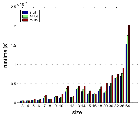
Fig. 18. Runtime performance (lower is better) of various DFTs of sizes between 3 and 64. For each size, the rightmost, middle, and leftmost bar shows (fixed point) code using multiplications and 14-bit and 8-bit multiplierless code, respectively. Platform: ipaq-0.4-lin.
