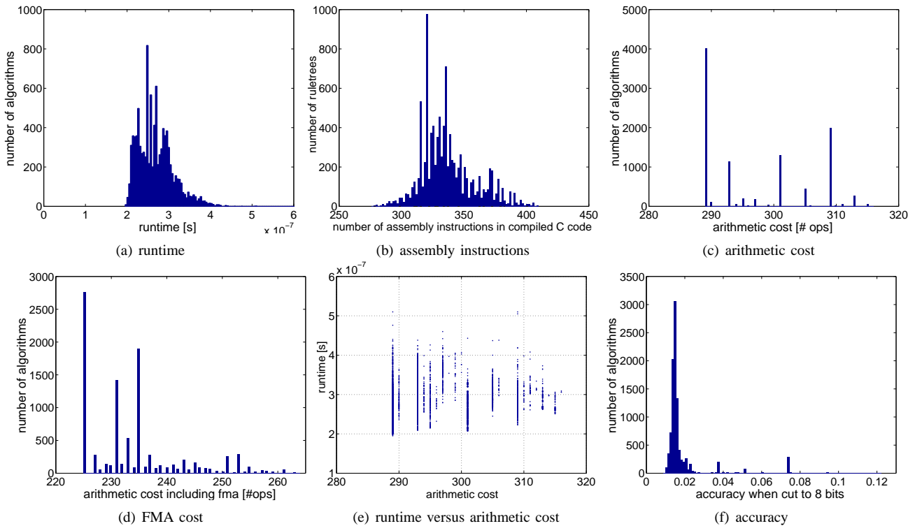
Fig. 8. Histograms of various data for 10,000 random fast formulas for a DCT-2 32 . From left to right: a) runtime; b) number of assembly instructions in the compiled C code; c) arithmetic cost; d) FMA optimized arithmetic cost; e) runtime versus arithmetic cost. f) accuracy when cut down to 8-bit fixed point; Platform: p4-3.0-lin.
