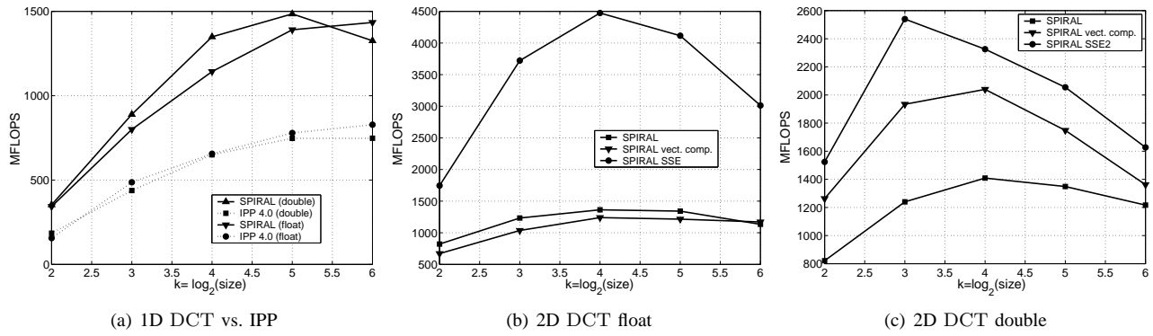
Fig. 12. (a) Comparing the performance (in MFLOPS) of SPIRAL generated code and IPP for a DCT-2 of size 2^k , 2 \leq k \leq 6 for single and double precision. (b) and (c) 2D-DCT float and double precision: scalar SPIRAL code, scalar SPIRAL code compiler vectorized, and SPIRAL vector code. Platform: p4-3.0-win.
