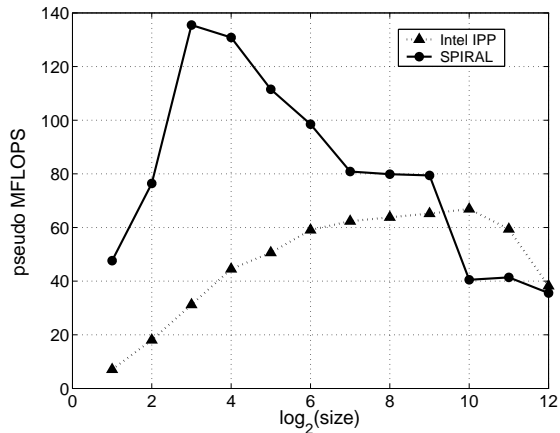
Fig. 11. Performance of SPIRAL generated fixed-point DFT code for sizes 2^1 – 2^{12} , on IPAQ vs. Intel IPP 3.0. Platform: ipaq-0.4-lin.
