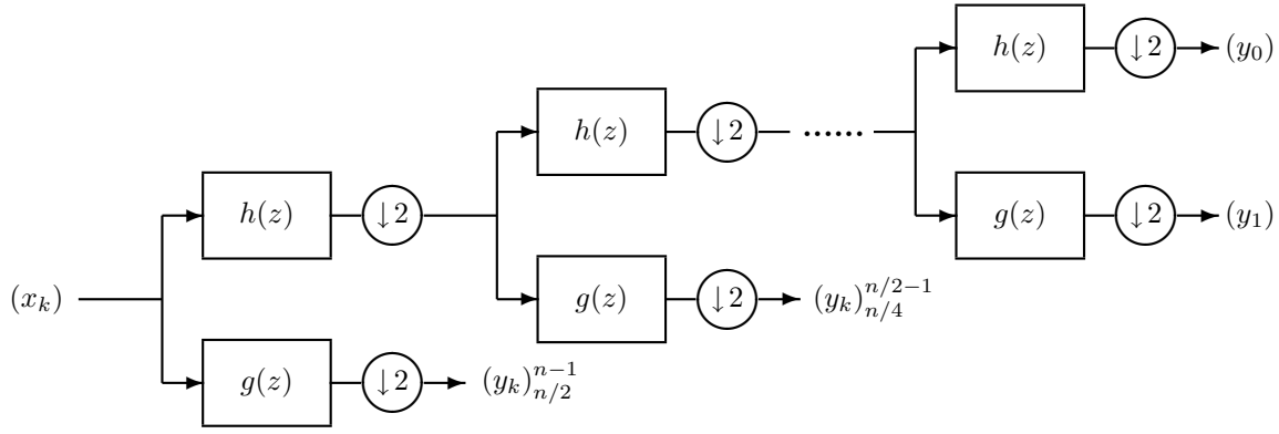
Fig. 2. Filter bank interpretation of the DWT.
