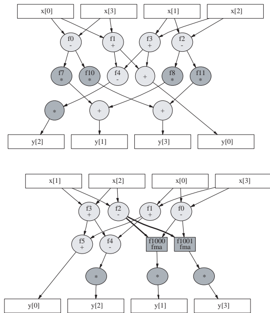
Fig. 5. Standard and FMA data flow graphs generated by SPIRAL for formula (41). Multiplications are shaded dark gray, FMAs are shown as dark gray rectangles.
