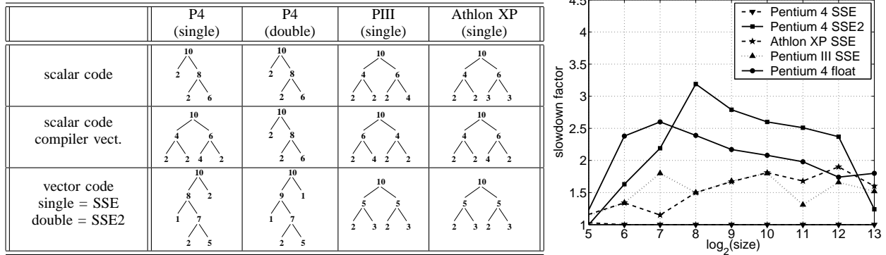
Fig. 15. Left: The best found DFT formulas for n = 2^{10} , represented as breakdown trees; right: crosstiming of best DFT ruletree, sizes 2^5, \dots, 2^{13} , generated for various platforms, implemented and measured on Pentium 4 using SSE. Platforms: p4-2.53-win, p3-1.0-win, xp-1.73-win.
