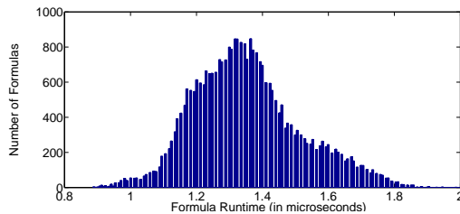
Fig. 3. Histogram of running times for all 31,242 \text{DCT}^{(IV)} , size 2^4 , formulas generated by SPIRAL's formula generator on a Pentium III running Linux.
