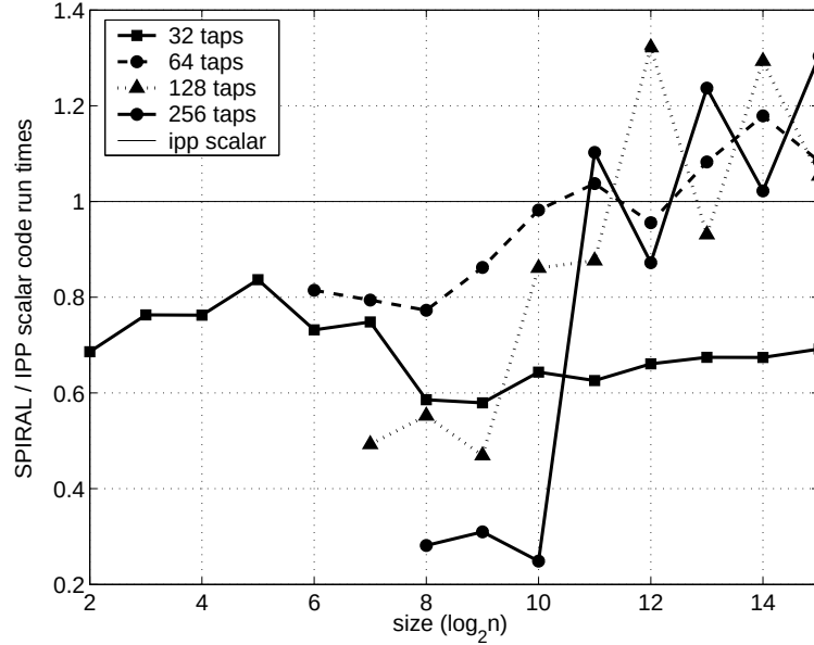
Figure 7.3: Comparing the best found filter code and IPP filter code on P4B-3.0-win
