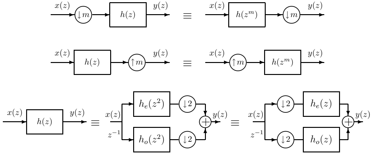
Figure 3.7: Noble identities (top); Efficient filtering using the Noble identity (bottom).
