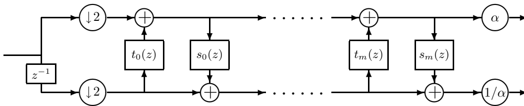
Figure 3.10: Lifting scheme for one stage of the forward DWT.
