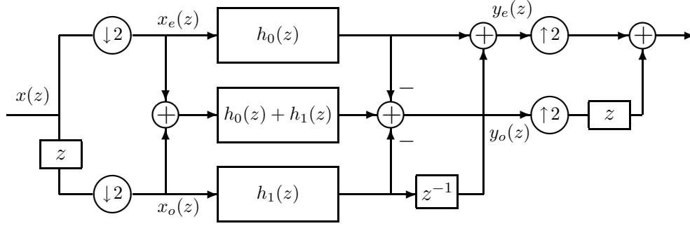
Figure 3.2: Radix-2 divide-and-conquer single step filter decomposition
