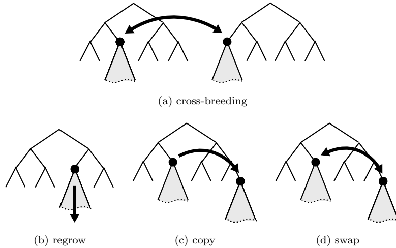
Figure 2.4: Rule tree manipulation for the evolutionary search: (a) cross-breeding; (b)–(d) three types of mutations: regrow, copy, and swap. †
