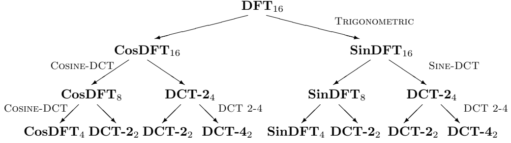
Figure 2.3: A \text{DFT}_{16} rule tree
