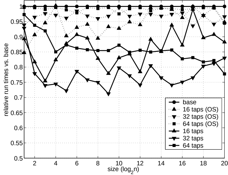
Figure 7.7: Comparison of the time-domain methods on Xeon-1.7 (lower is better)
