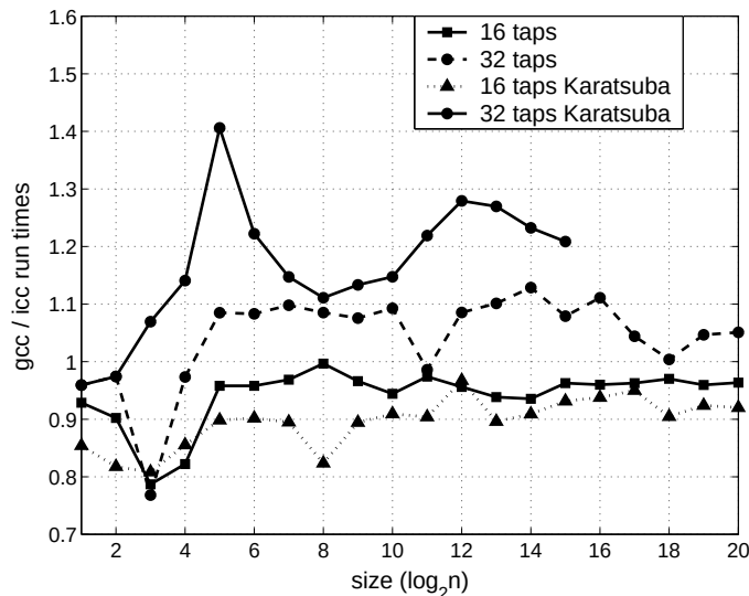
Figure 7.13: Comparison of run times for time-domain and Karatsuba methods compiled by icc-8.0-lin and by gcc-O1-3.3 compilers on P4-1.6-lin platform
