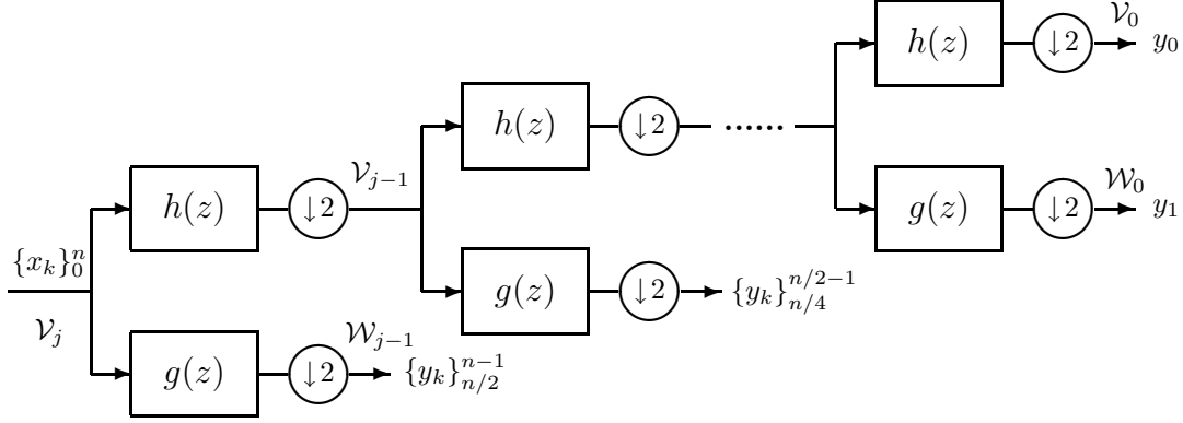
Figure 3.3: Filter bank interpretation of the DWT.
