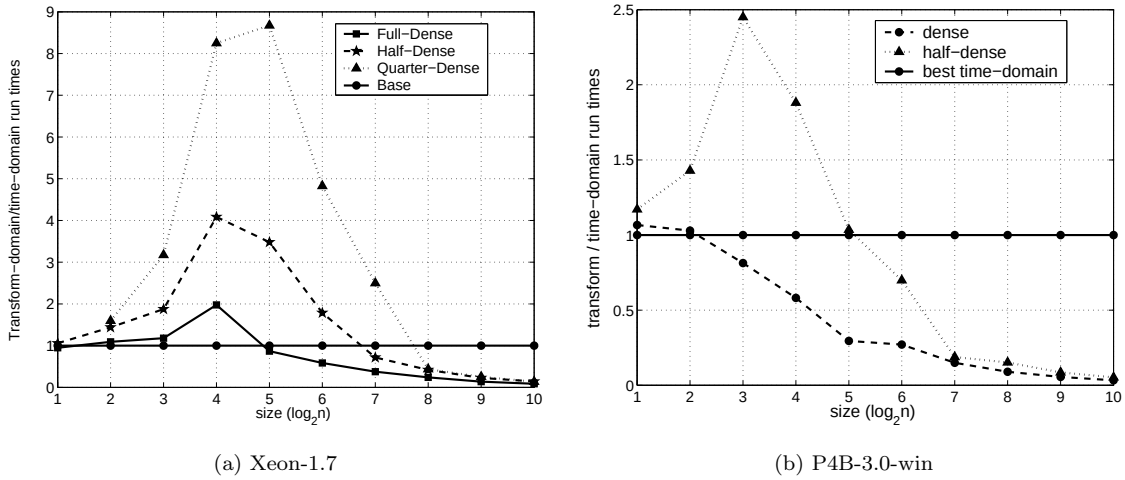
Figure 7.12: Comparison of time-domain and transform-domain methods for circulant matrices.
