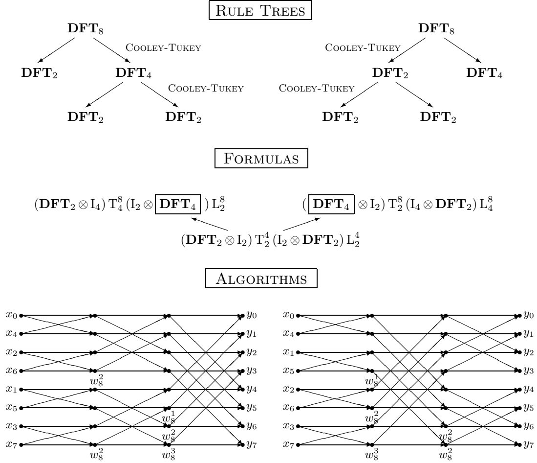
Figure 2.2: Rule trees = formulas = algorithms.
