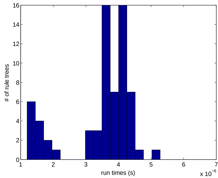
Figure C.1: Runtime comparison of all lifting scheme factorizations for Daubechies 9/7 wavelet transform
