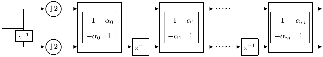
Figure 3.9: Lattice decomposition of an orthogonal filter bank.
