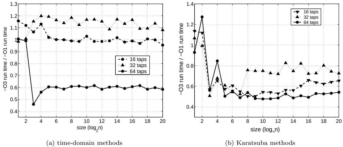
Figure 7.14: Effect of compiler options gcc-mac-O1 and gcc-mac-O3 on the run time of: (a) time-domain methods, and (b) Karatsuba methods for filters on Macintosh platform.
