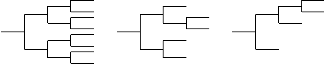
Figure 3.5: Wavelet packet trees: full (left); pruned (center); DWT (right).
