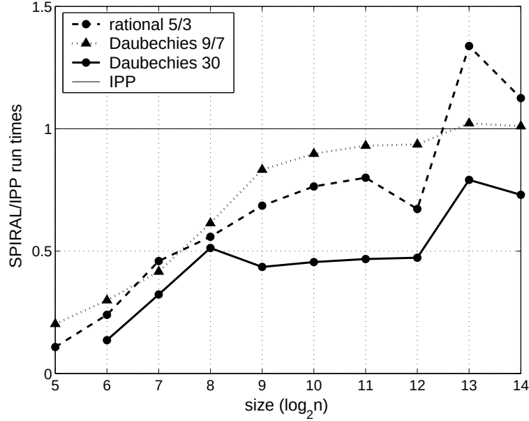
Figure 7.2: Comparing the best found DWT implementation and IPP code on Athlon-1.73 (lower is better)
