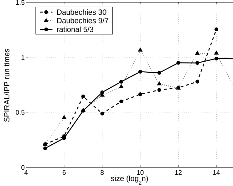
Figure 7.4: Comparing the best found DWT code and IPP DWT code on P4B-3.0-win for three wavelets: rational 5/3, Daubechies 9/7, and Daubechies 30
