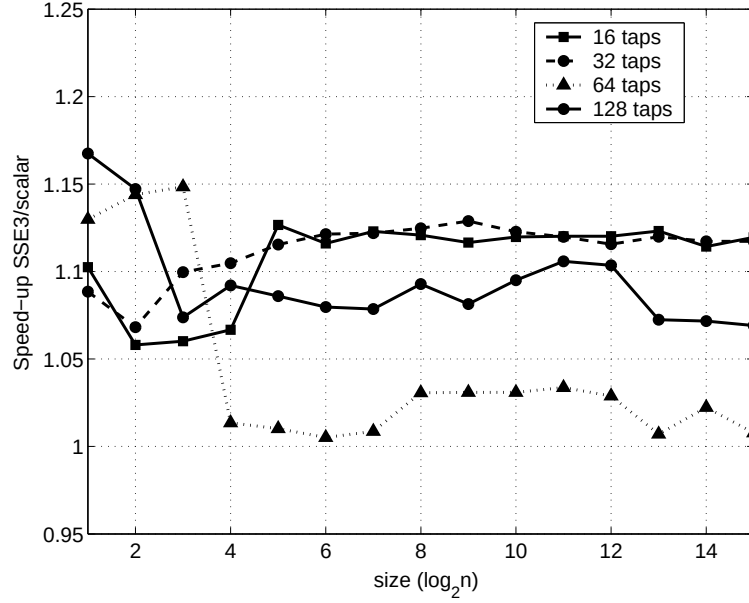
Figure 7.15: SSE3 vectorization speedup for FIR filters obtained by Intel-SSE3 compiler
