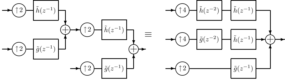
Figure 6.2: Computing synthesis channel filters using Noble identities.
