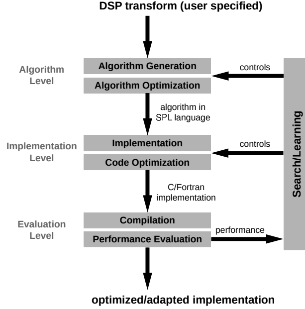
Figure 2.1: The architecture of SPIRAL
