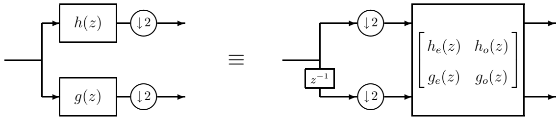
Figure 3.8: Polyphase representation of one filter bank stage.
