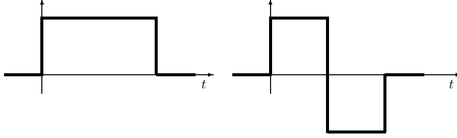
Figure 3.6: Haar scaling function and the wavelet.
