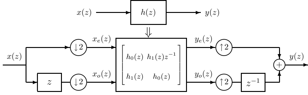
Figure 3.1: Filtering interpreted as polyphase filtering with two channels.
