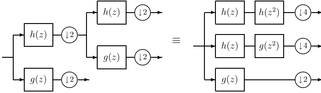
Figure 6.1: Computing channel filters using the Noble identities.
