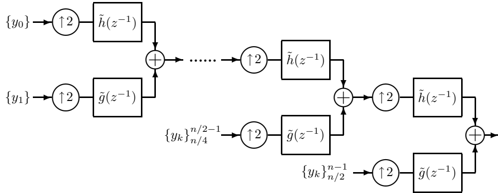
Figure 3.4: Filter bank representation of the inverse DWT.
