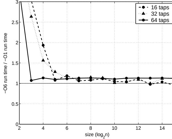
Figure 7.8: Blocking methods for gcc-O6-3.2 and gcc-O1-3.2 on Xeon-1.7
