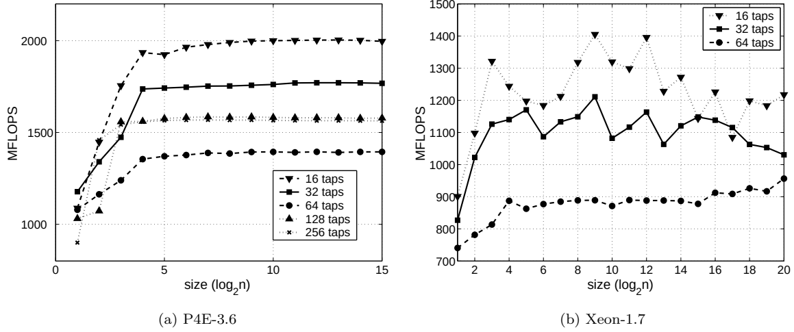
Figure 7.9: Performance in MFLOPS for best found time-domain method.
